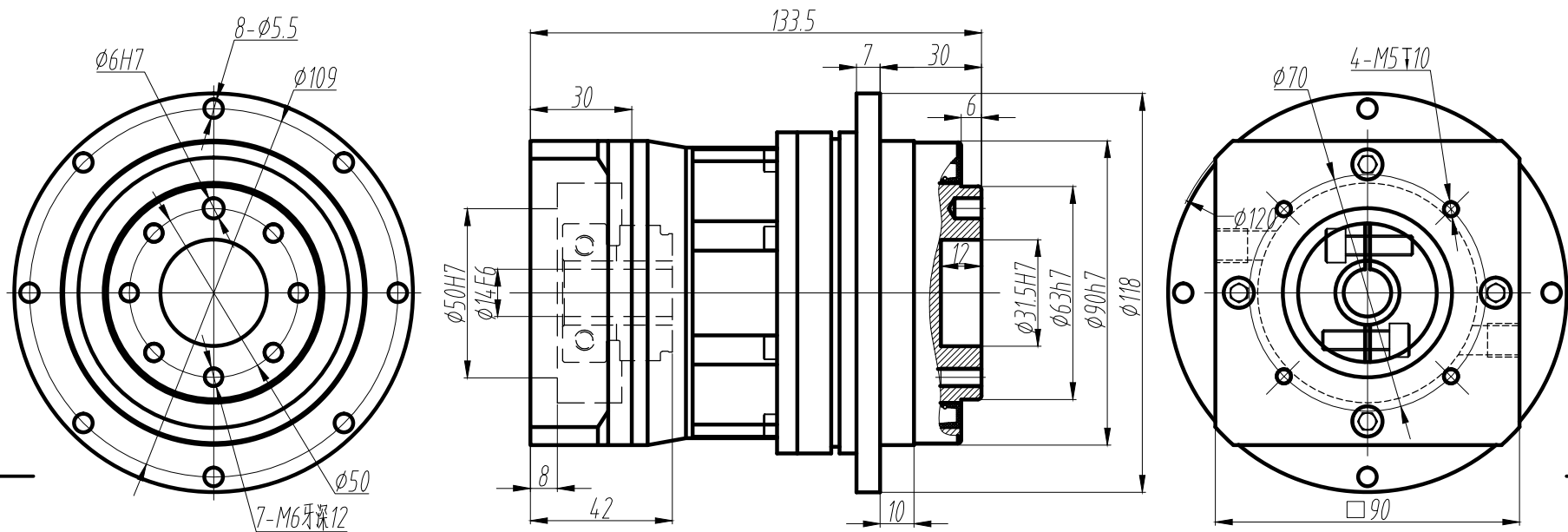
标准轴 Standard output shaft
